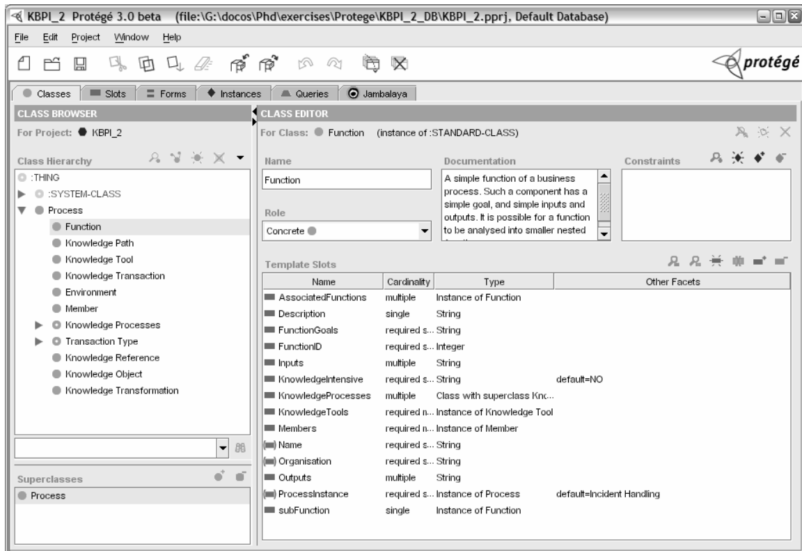
Figure 8: Protégé displaying details of the Function class
