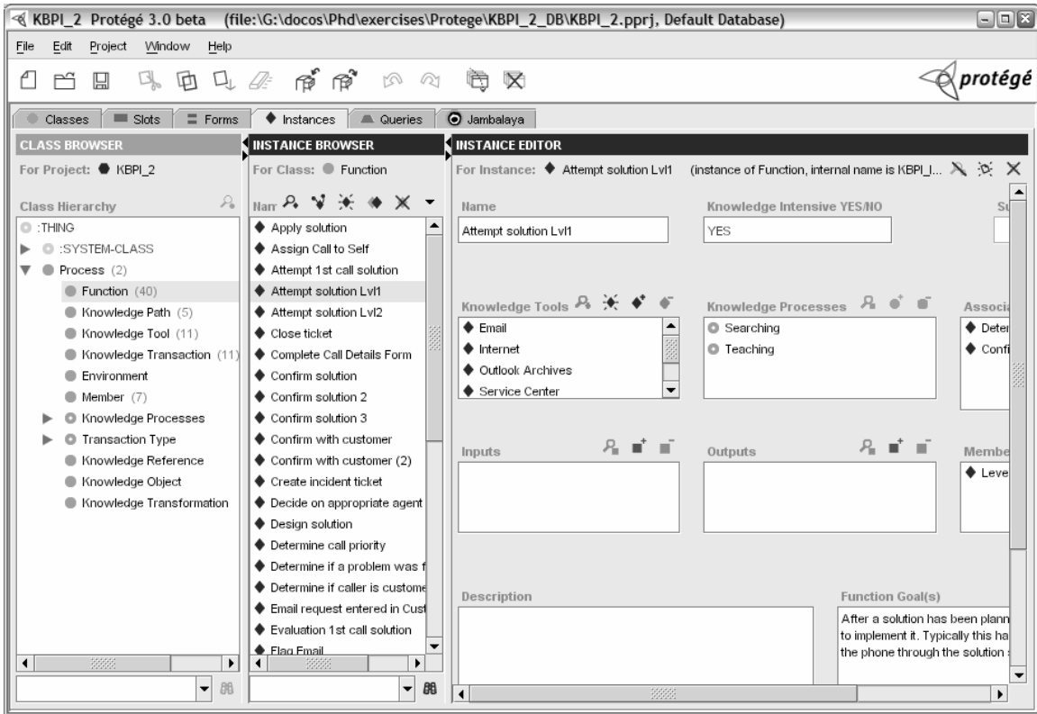
Figure 9: Protégé displaying instances of the Function class
